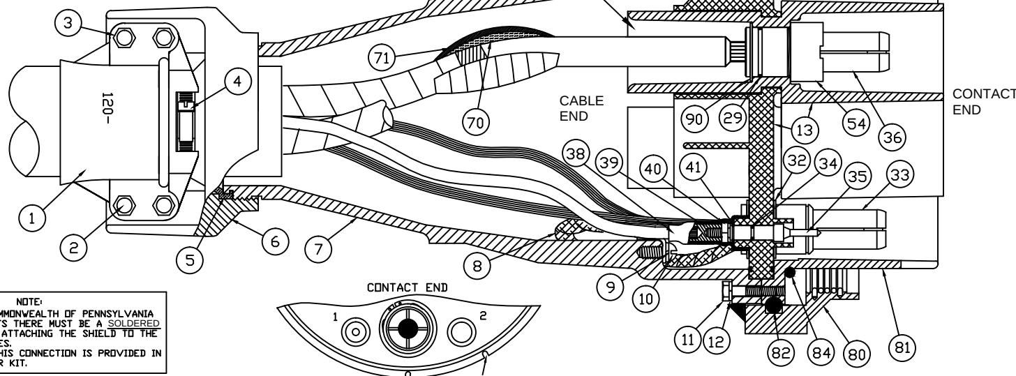
FIGURE 1 INSERT ROLL PIN INTO THIS SLOT
